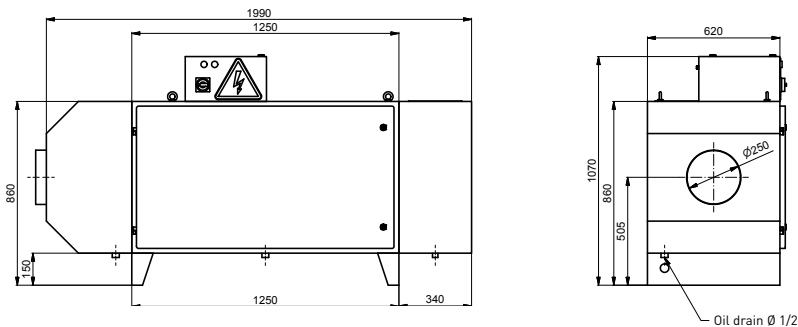
Side and frontal view tandem individual filter B 3000 EFT
