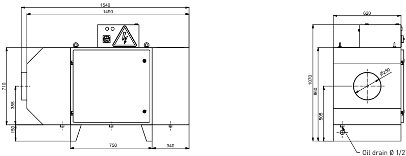
Side and frontal view individual filters B 3000 EF | B 3000 MF
