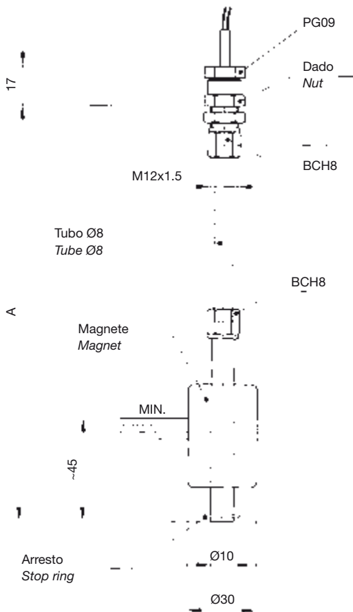
LM2P SPDT CONTACT
